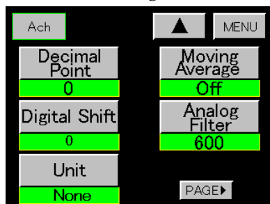
Itemized setting screen 4/5
