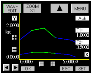
HI/LO limit waveform set-value
