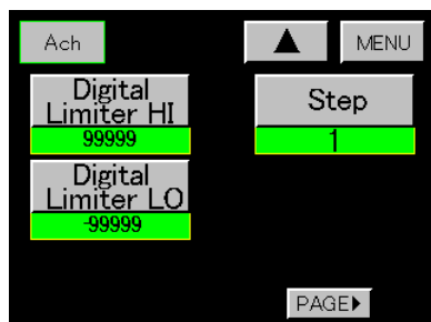
Itemized setting screen 5/5
