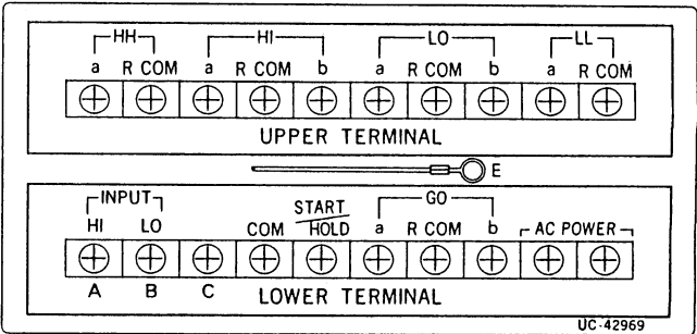
Fig. 5 4.2 Terminal Connection
