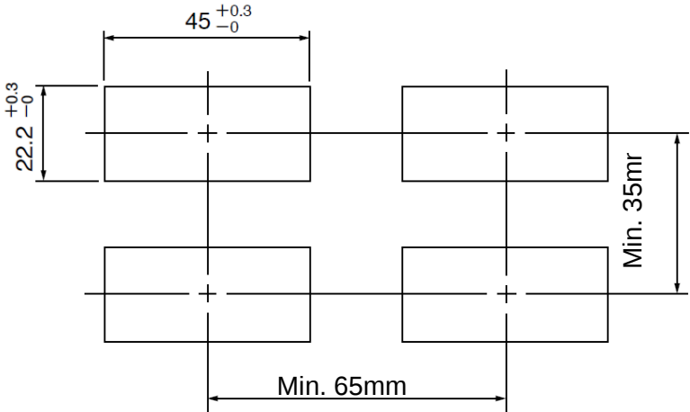
◆Panel cutout
